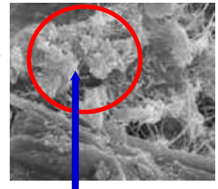
Transformation to Calcium Silicate Hydrate and other organic compound.
